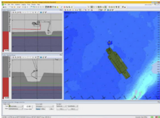
Trimble Marine Construction software for excavator dredge application - alternative view
